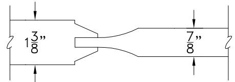
TYPE 'B' STICKING WITH 'SC1' PANEL
