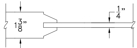
TYPE 'B' STICKING WITH 'F1' PANEL
