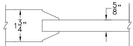
TYPE 'B' STICKING WITH 'F2' PANEL
