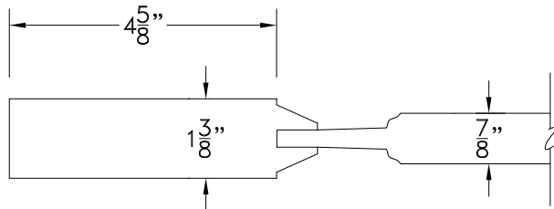
TYPE 'B' STICKING WITH 'A1' PANEL
